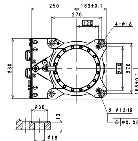
Installation Dimensions
