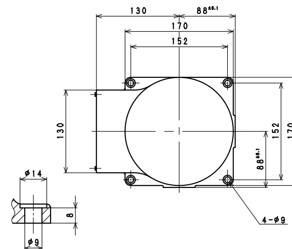
Installation Dimensions
