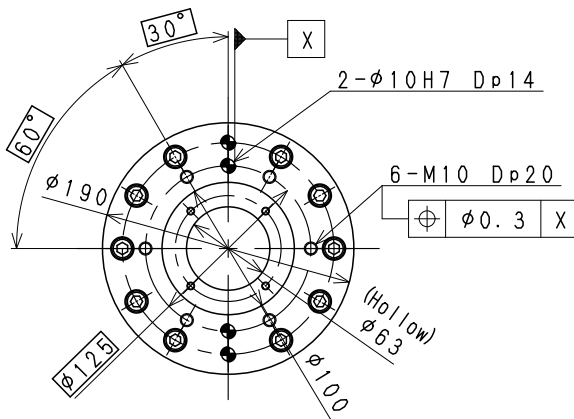
OPTION FLANGE
