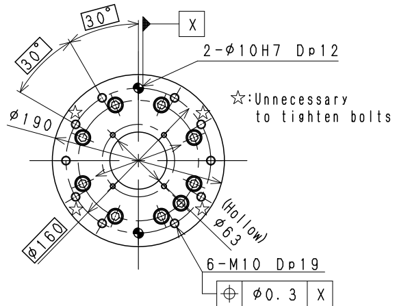
STANDARD FLANGE
