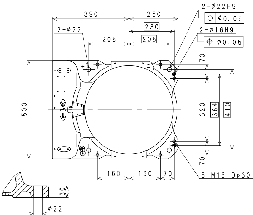
Installation Dimensions
