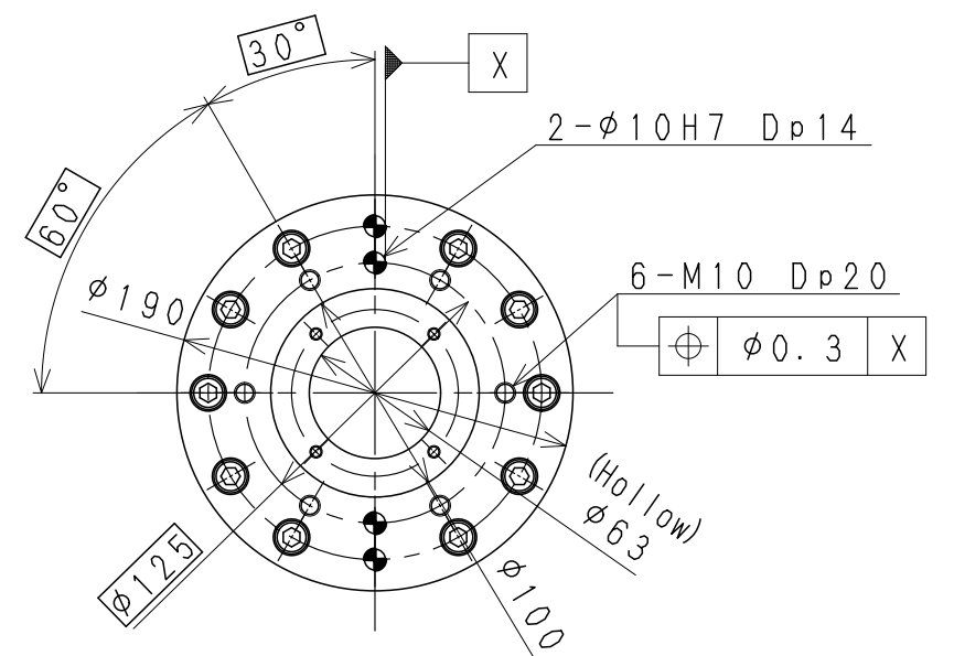
OPTION FLANGE
