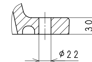
Installation dimensions
