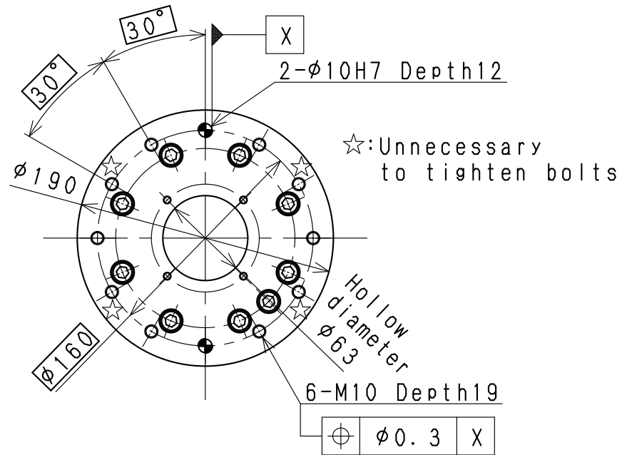
STANDARD FLANGE
