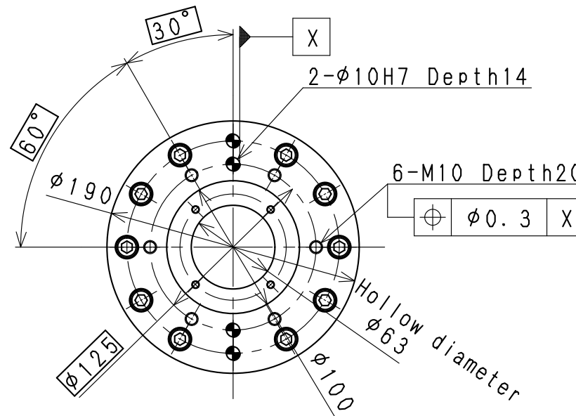
OPTION FLANGE
