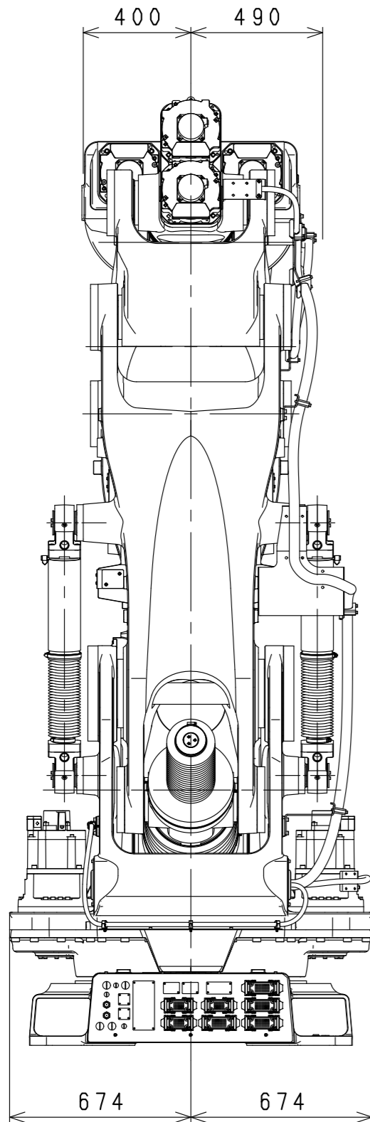
Installation Dimensions
