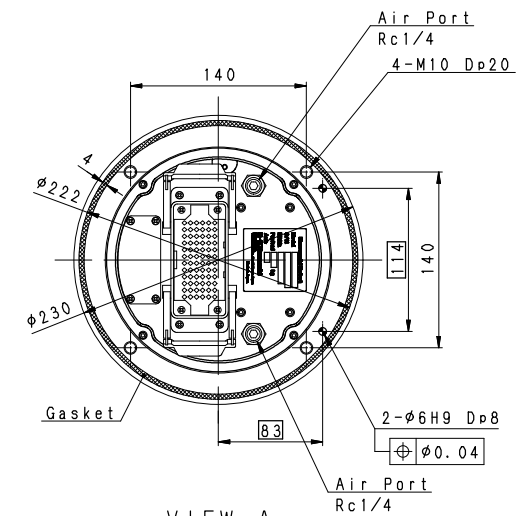
VIEW A (Installation Dimensions)
