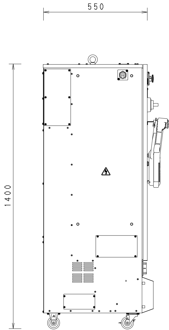
SIDE VIEW
