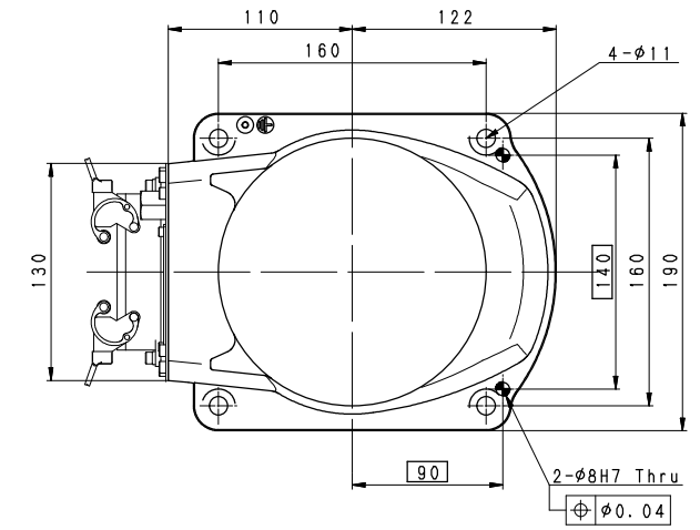
Installation Dimensions
