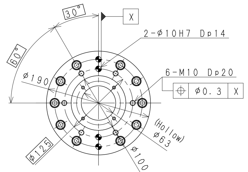
OPTION FLANGE
