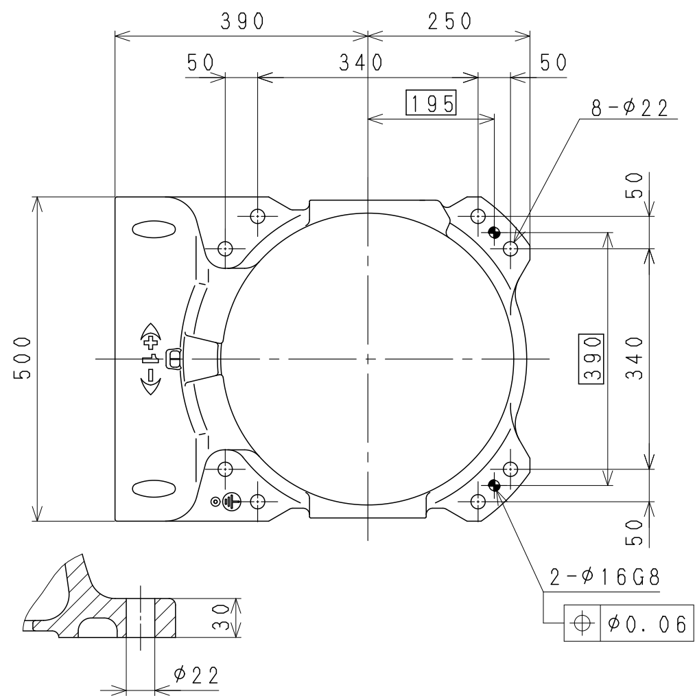
Installation Dimensions
