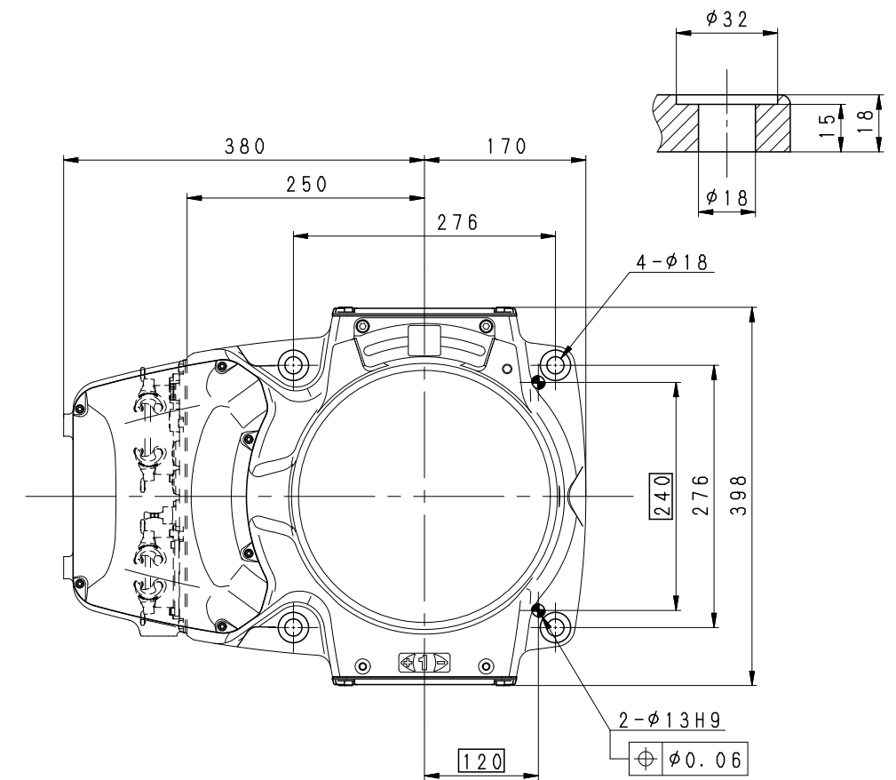
Installation Dimensions
