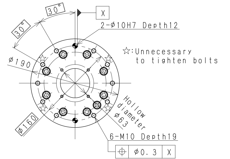
STANDARD FLANGE
