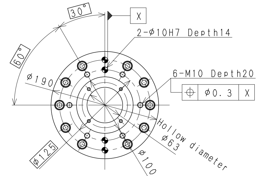
OPTION FLANGE
