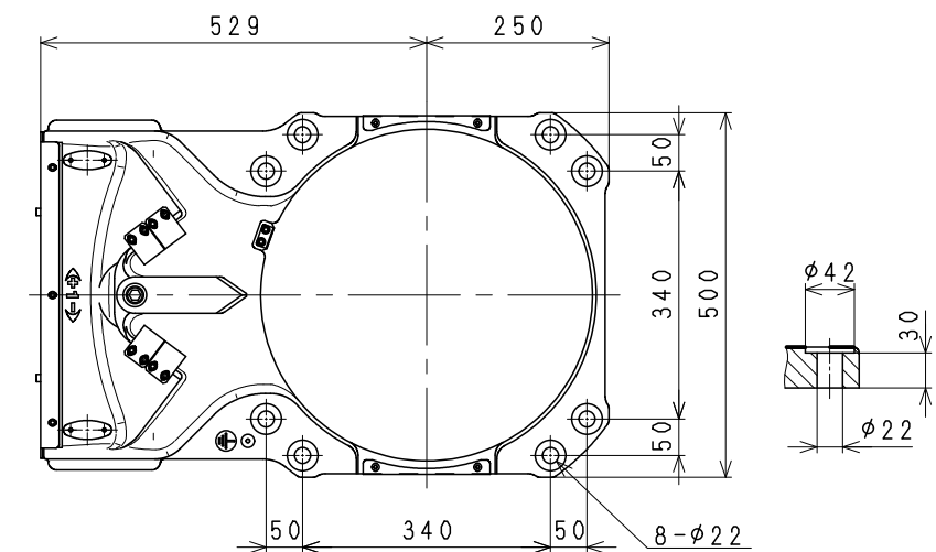
Installation dimensions
