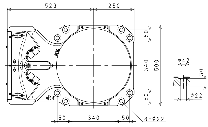
Installation dimensions
