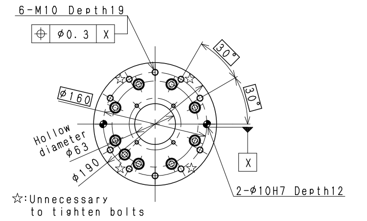
VIEW A
