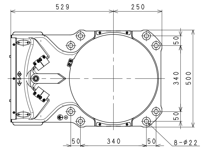
Installation dimensions
